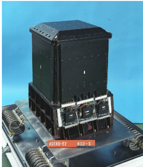
Fig. 1. Hard X-ray Detector before installation.
