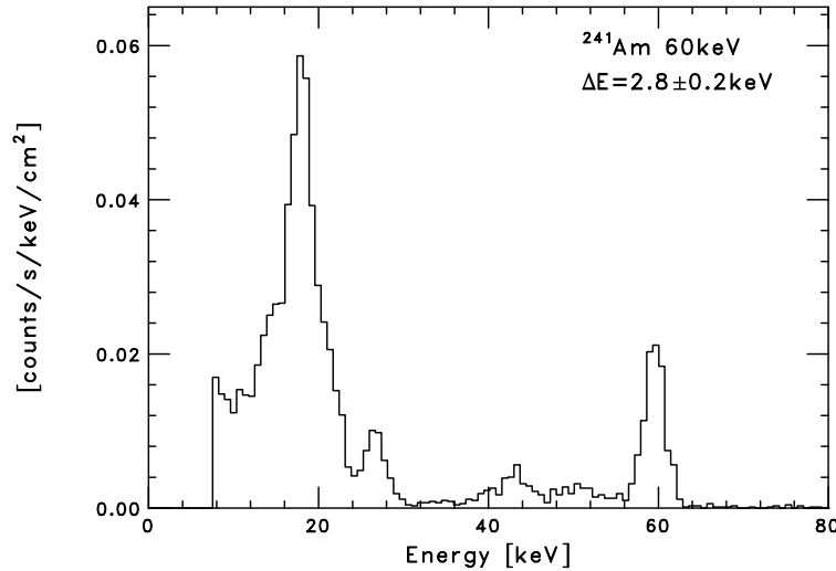
Fig. 14. PIN spectrum of ^{241}\text{Am} obtained at -20^{\circ}\text{C} .
