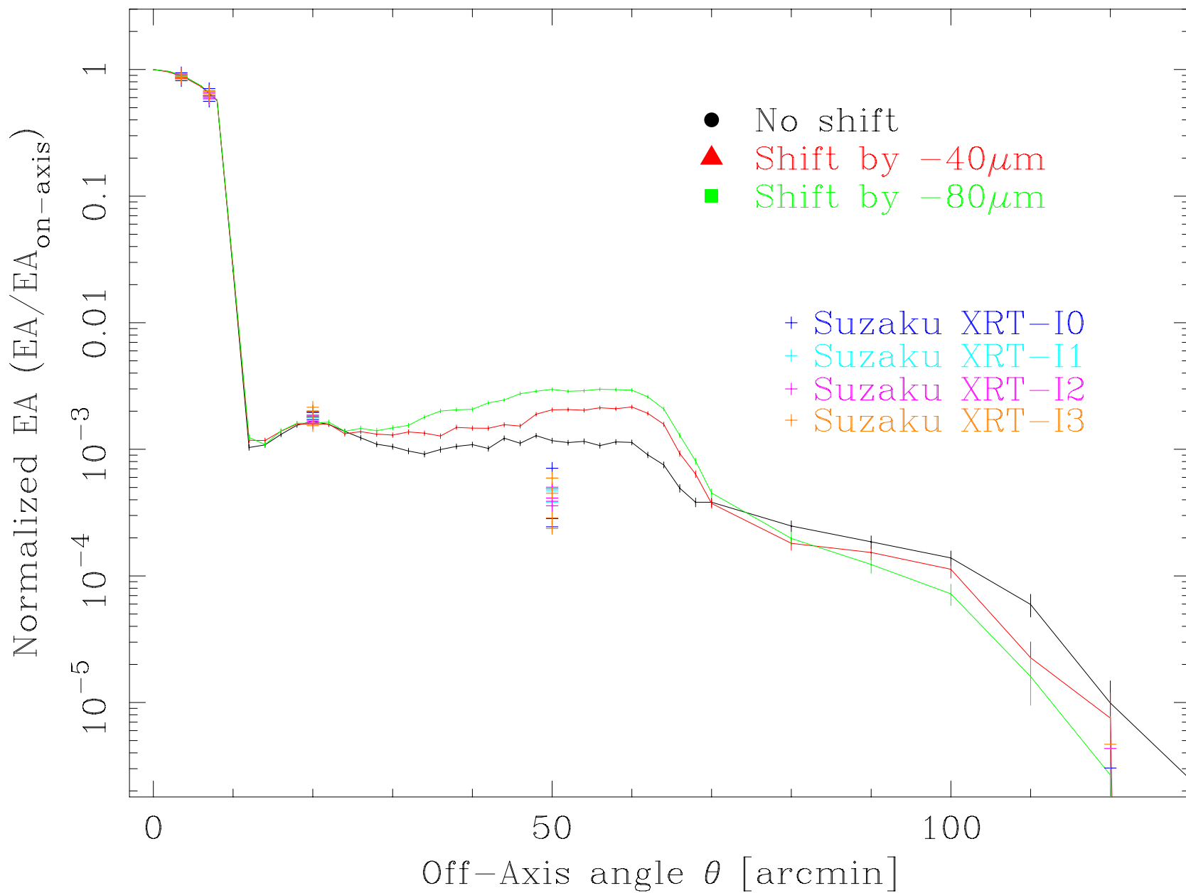
Angular response of XRT stray E.A. (Al-K \alpha : 1.49keV)
