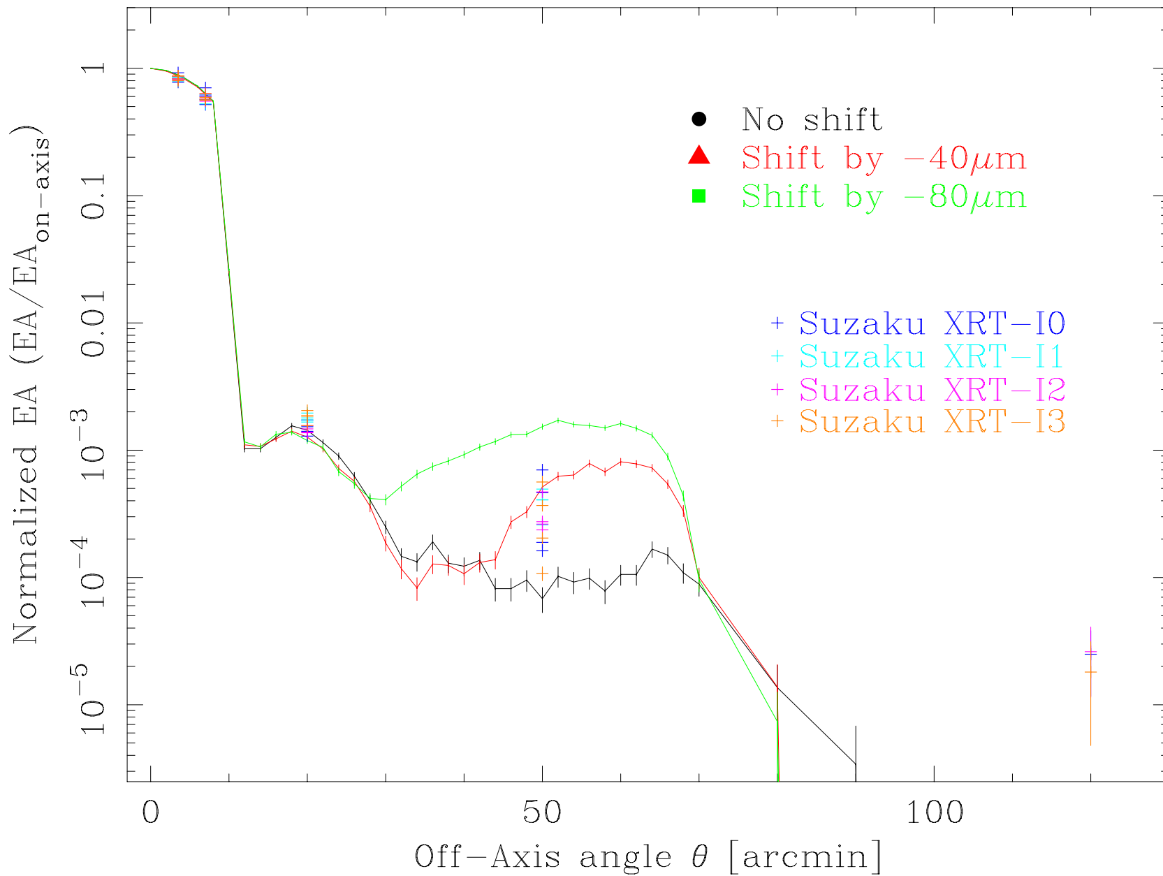
Angular response of XRT str A. (Ti-K \alpha : 4.51keV)
